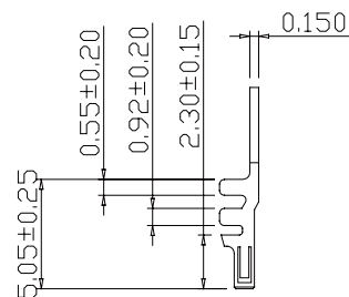
PartNo.: 1255-T-L
