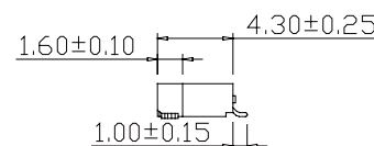
PartNo.: 1255MR-XXGB-U
